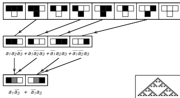
rule 90
