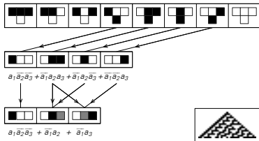
rule 30
