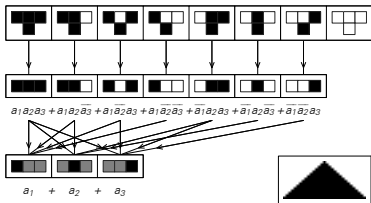
rule 254
