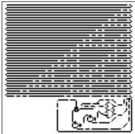
rule 110
