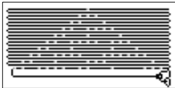
rule 30
